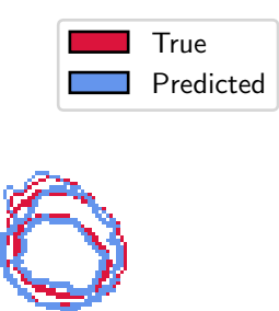
segmentations
